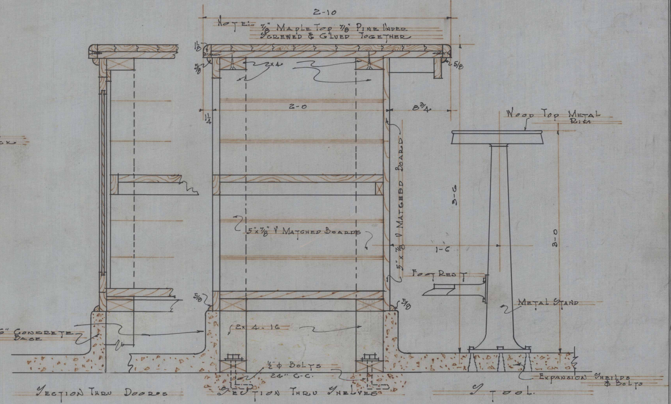
DETAILS OF COUNTER IN LUNCH ROOM Scale 1/2"=1'-0"
