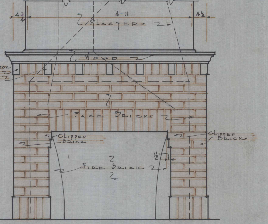
ELEVATION OF RECEPTION ROOM FIREPLACE
