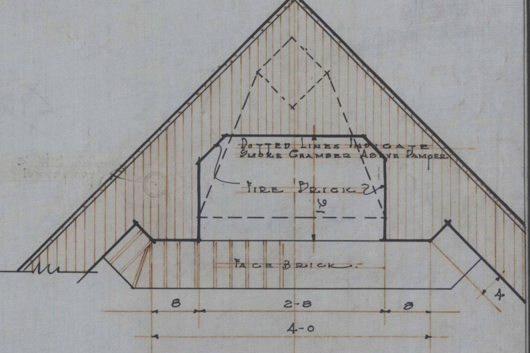
PLAN
