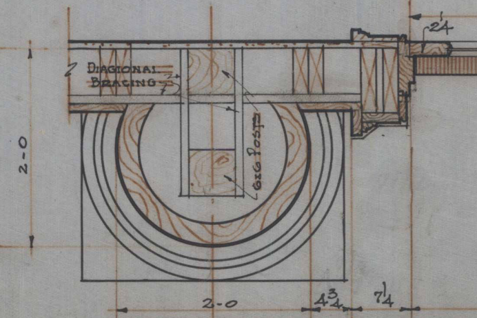
TYPICAL DETAIL FOR ENGAGED COLUMNS
