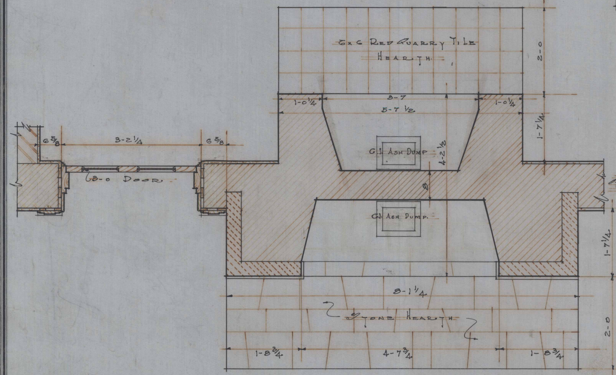
PLAN
