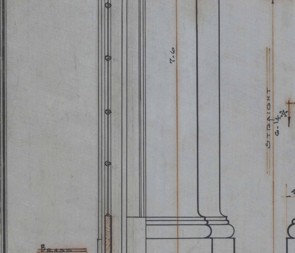
SECTION THIRD OF FRONT DOORS - SECTION C-C - SCALE 2 1/2" = 1'-0"
