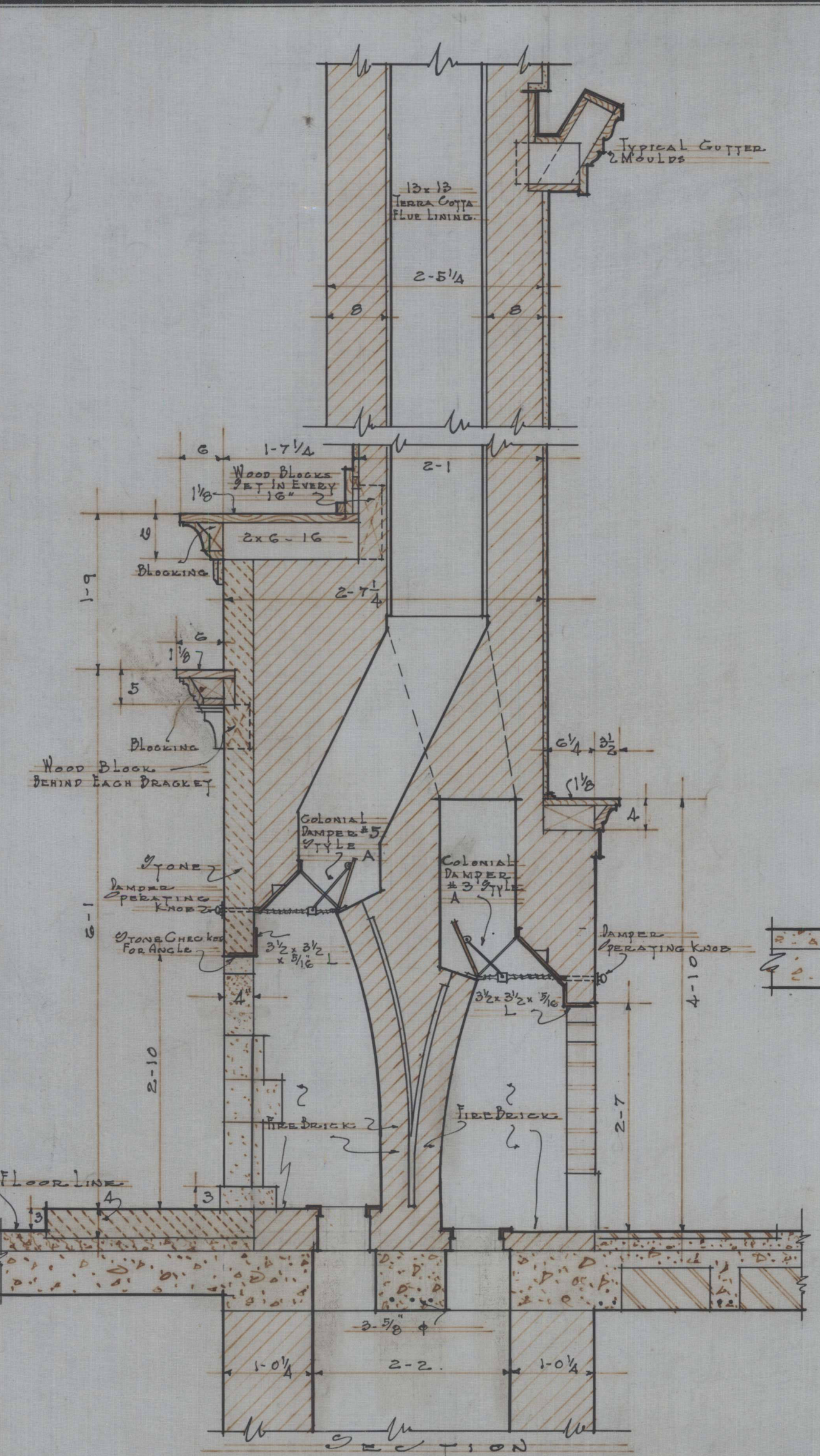
SECTION
