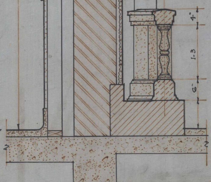
SECTION THIRD OF STUCCO PANEL - B-B
